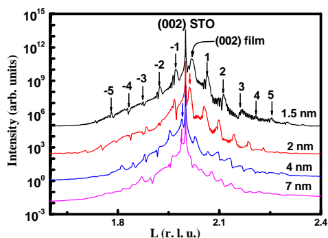
Fig. 3. Intensity distribution of a (002) radial scan spectrum of LCMO/LNO superlattice films.
