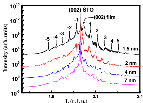
Fig. 3. Intensity distribution of a (002) radial scan spectrum of LCMO/LNO superlattice films.
